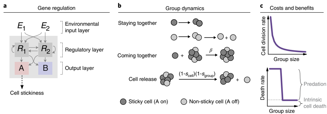
Fig. 1 | Overview of the model. a , Each cell is equipped with a gene regulatory network that senses the environment. A, B, R_1, R_2 denote genes; E_1 and E_2 denote environmental factors. Environment 1 is specified by E_1 = 1, E_2 = 0 ; environment 2 is specified by E_1 = 0, E_2 = 1 . The optimal expression pattern in environment 1 is to express only gene A; the optimal expression pattern in environment 2 is to express only gene B. Deviations from these optimal expression patterns lead to a 70% (if one gene has the incorrect expression status) or 90% (if both genes have the incorrect expression status) decrease in reproduction. Cell stickiness arises as a promiscuous function of gene A. b , Mechanisms of group formation and disintegration (see Methods for details and Table 1 for parameters). The probability to dissociate (1 - s_{\text{cell}})(1 - s_{\text{group}}) depends on cell stickiness s_{\text{cell}} and group stickiness s_{\text{group}} , which is simply the mean stickiness of all group members. c , Costs and benefits of group formation. Cells in sufficiently large groups (size at least k ) have a survival advantage because they incur no mortality due to predation.
