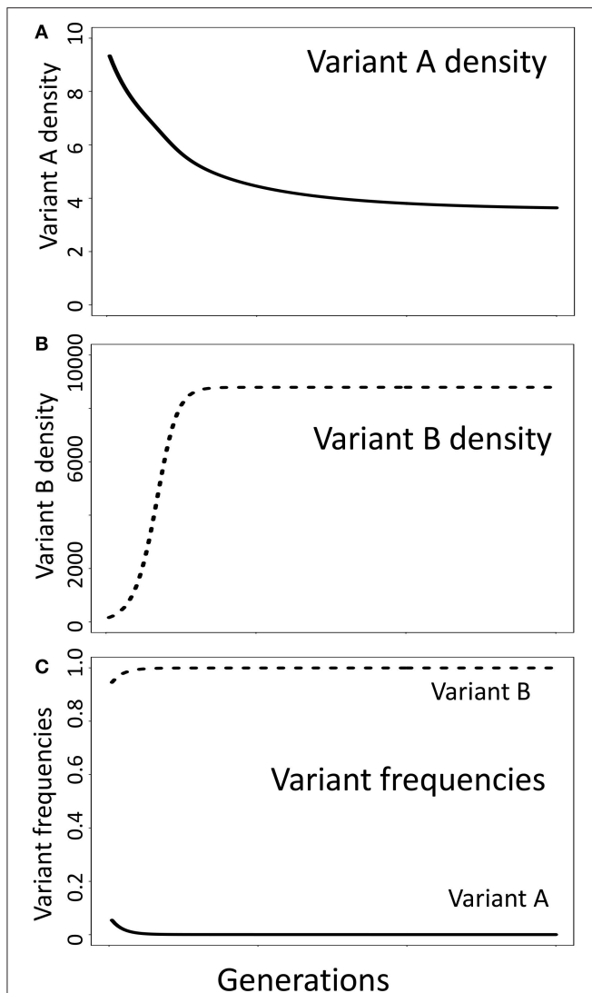
FIGURE 2 | Multi-niche selection, an alternative model of balancing selection, does not require the core assumption of negative frequency-dependent selection models that relative fitness is a function of relative frequency in the population. Shown is a simulation where variant A has a selective advantage in niche A while variant B has a selective advantage in niche B (Appendix 1, Supplementary Material). Here, the carrying capacity in niche A is much lower than in niche B ( K_A = 10 , K_B = 10,000 ). At the start of the simulation, there are 10 variant A individuals (10% of the population) and 90 variant B individuals (90% of the population), yet the fitness (growth rate) of variant A individuals is much lower than for variant B individuals. This contradicts the expectations of negative frequency-dependent selection, where the frequency of variant A should increase as it is currently less frequent than variant B. Although the conditions necessary for negative frequency-dependent selection to maintain a stable polymorphism are not satisfied, both variants can be maintained in the population due to the selective advantage each enjoys in their preferred niche. Parameters used in the simulation: growth rate = 0.35, death rate in preferred niche = 0.05, death rate in non-preferred habitat = 0.25, migration among niches = 0.01.
